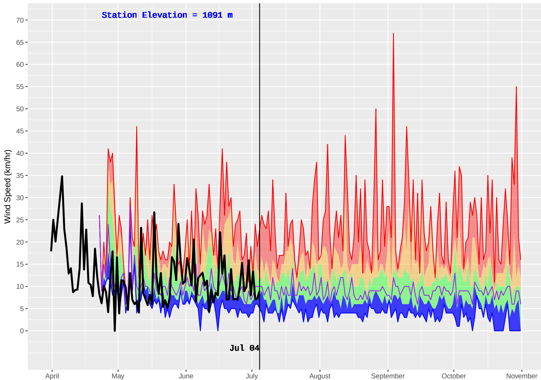
BIG MOUTH 2 (868) : Historical (2004–2016) and Current (2018) Noon Wind Speed
